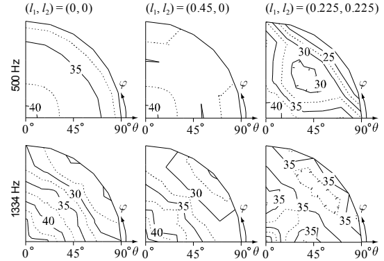
Fig. 4 Incidence angle dependence of transmission loss with/without niche at 500 Hz ( < f_c ) and 1334 Hz ( > f_c )
