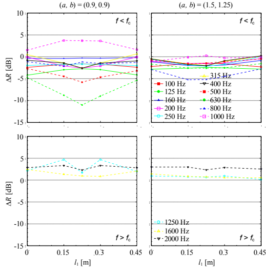
Fig. 6 Influence of the depth of two-sided niche on random-incidence transmission loss ( h_p = 10 [mm], \eta_s = 0.5 ).
