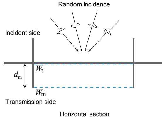
Fig. 8 Measurement surface setting.
