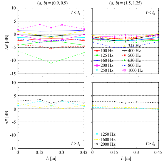
Fig. 7 Influence of the depth of two-sided niche on random-incidence transmission loss ( h_p = 10 [mm], \eta_s = 0.1 ).
