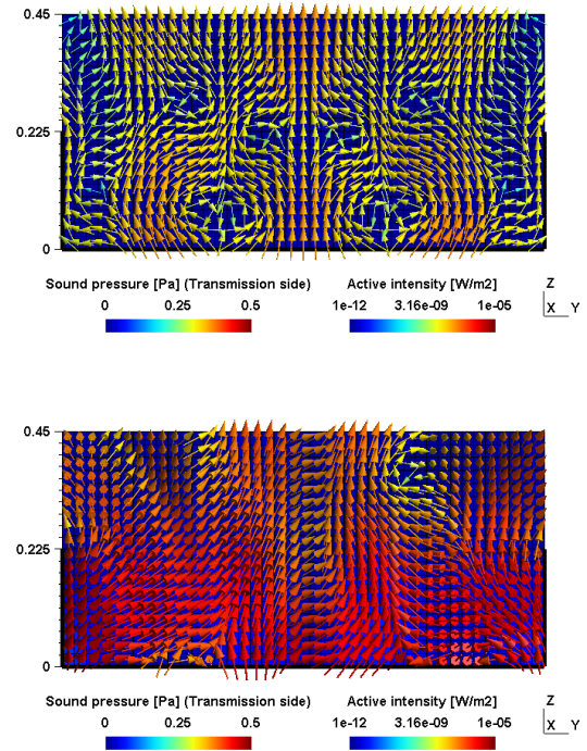
Fig. 10 Distributions of sound pressure
